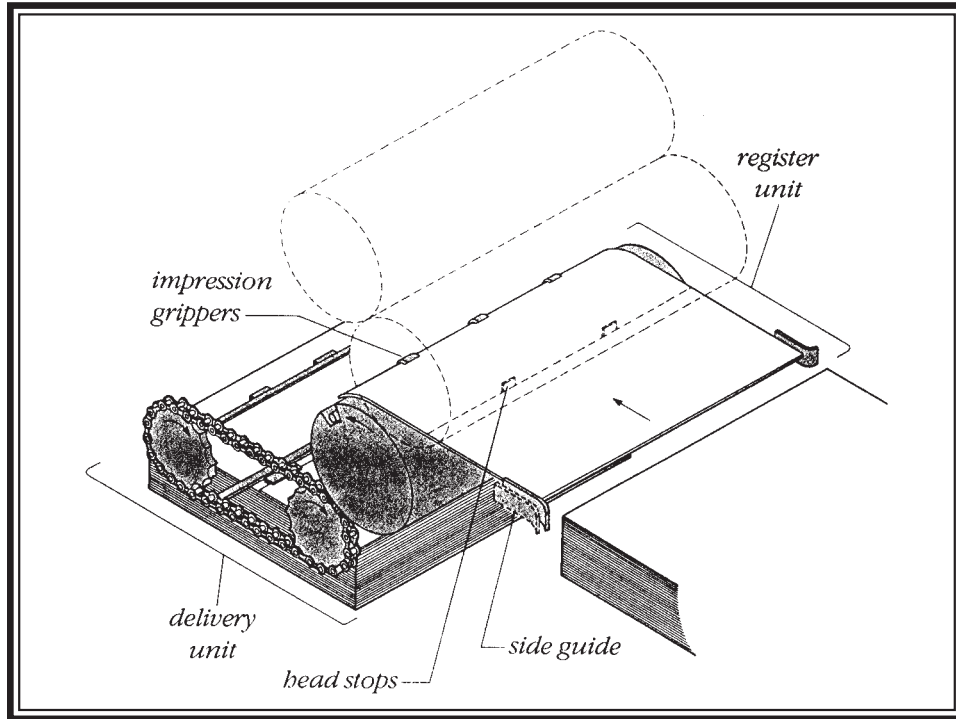
Sheet-fed offset-lithographic press register (sheet-control) system
