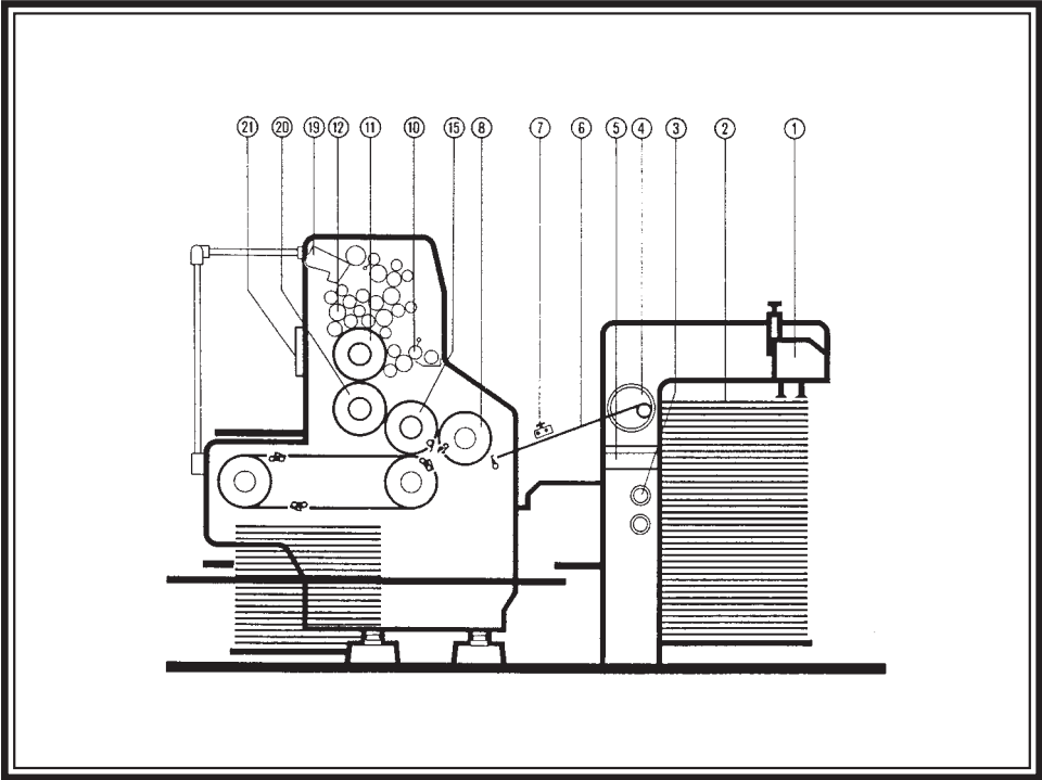
Schematic of single-color offset-lithographic press
