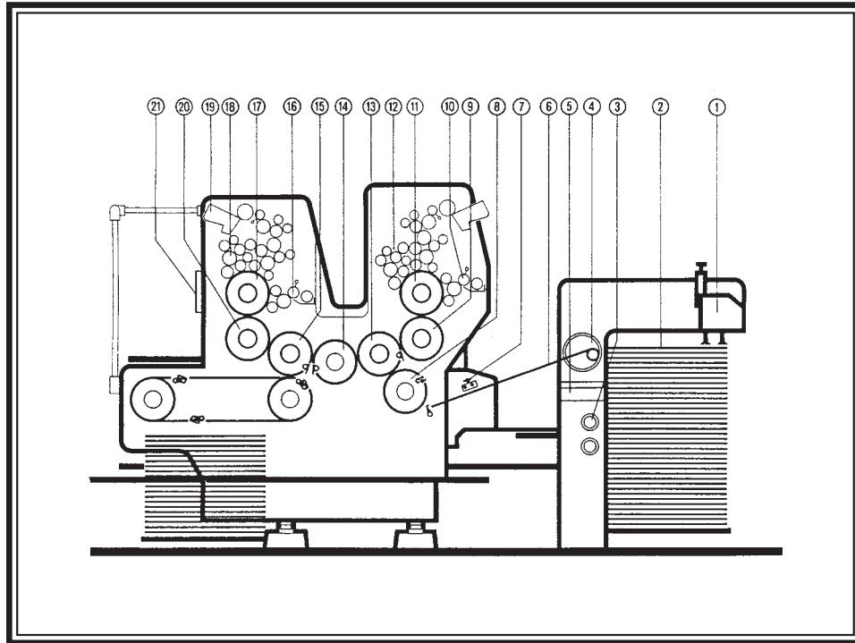
Schematic of two-color offset-lithographic press
